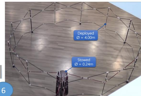
Outer ring structure of Large Deployable Antenna
